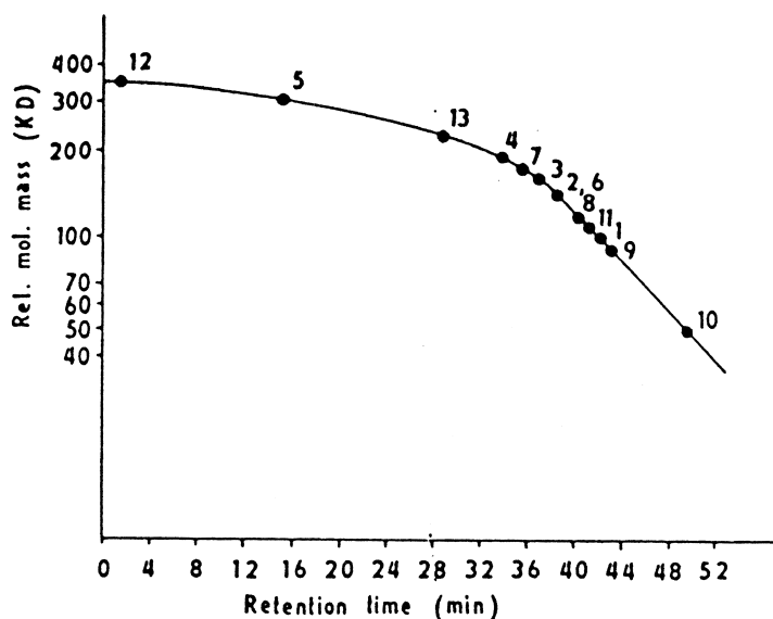
Fig. 5. Retention time vs. relative molecular mass relation for different collagen chains in the case of HPLC separation on Separon HEMA 1000 Glc column. For identification of chains see Table 2. Reprinted from Deyl et al. [43].
